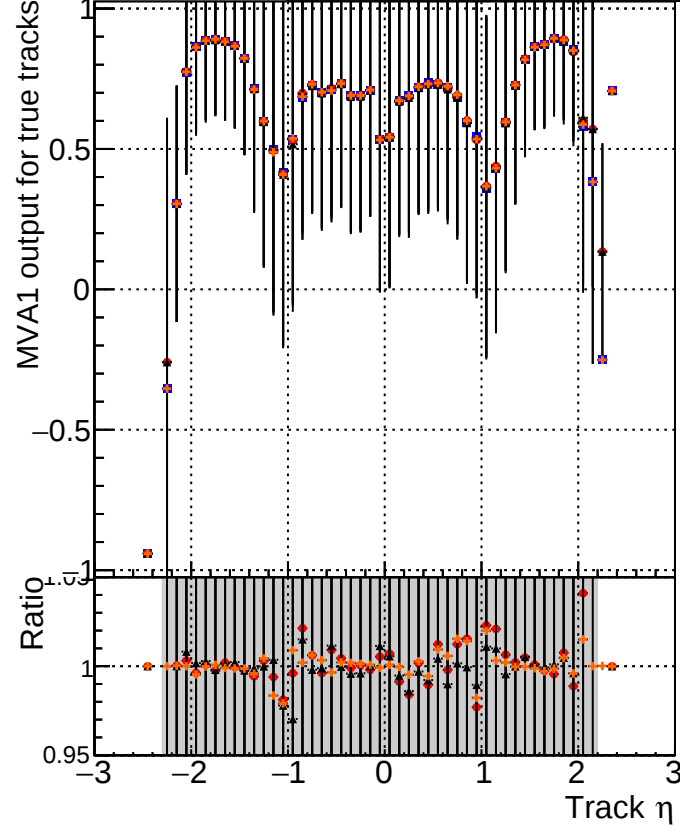
MVA1 of associated tracks (recoToSim) vs. track \eta Legend: \blacksquare DQM_mkFit_TToriginal \bullet DQM_mkFit_TTNEWHS \blacktriangledown DQM_mkFit_TTNEWHS-dpdq \blacktriangleright DQM_mkFit_TTNEWHS-chi2
