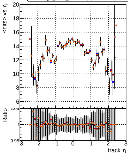
Legend: DOM_mkFit_TToriginal DOM_mkFit_TTNEUHS DOM_mkFit_TTNEUHS-dpdq DOM_mkFit_TTNEUHS-chi2 mean hit
