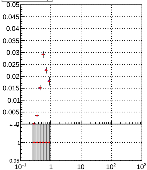
—•— /data2/legianni/JSON-bkwd-fwd/no-modif/CMSSW_13_0_X_2023-01-24-1100/src/DQM_original —•— DQM_modified
