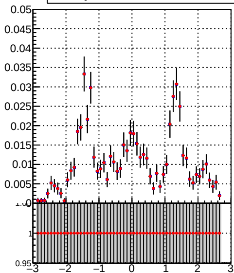
—•— /data2/legianni/JSON-bkwd-fwd/no-modif/CMSSW_13_0_X_2023-01-24-1100/src/DQM_original —•— DQM_modified
