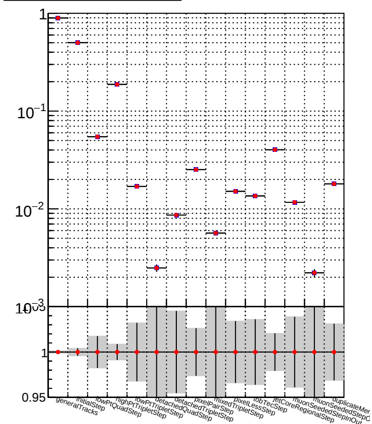
Duplicates rate vs collection Legend: - /data2/legianni/JSON-bkwd-fwd/no-modif/CMSSW_13_0_X_2023-01-24-1100/src/DQM_original (grey bar) - DQM_modified (red line with square markers)
