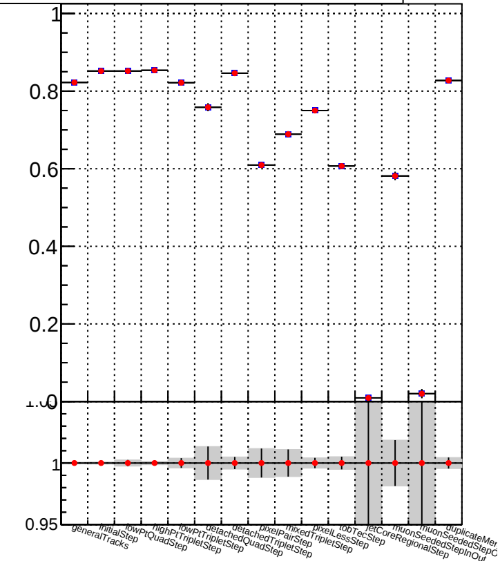
Duplicates rate vs collection Legend: - /data2/legianni/JSON-bkwd-fwd/no-modif/CMSSW_13_0_X_2023-01-24-1100/src/DQM_original (grey bar) - DQM_modified (red line with square markers)
