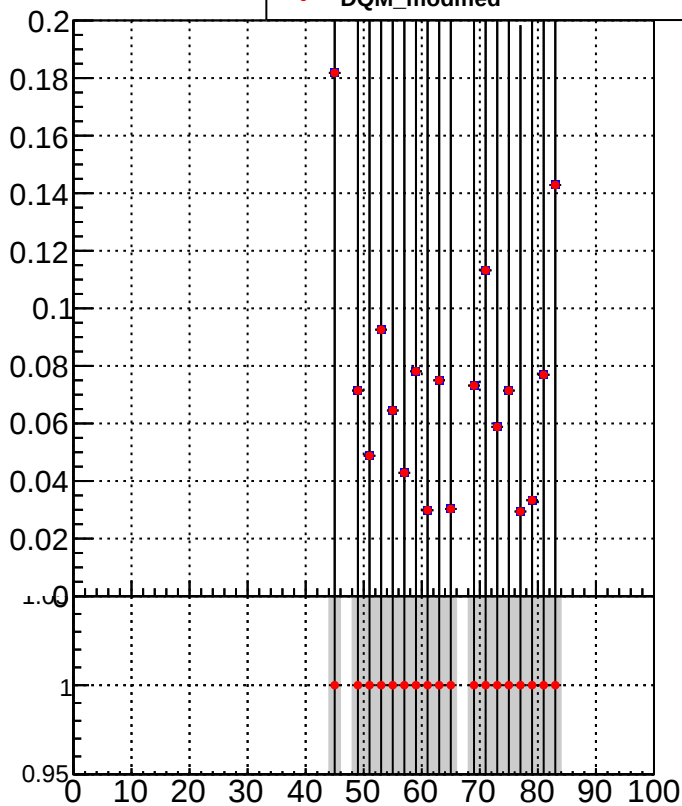
/data2/legianni/JSON-bkwd-fwd/no-modif/CMSSW_13_0_X_2023-01-24-1100/src/DQM_original DQM_modified
