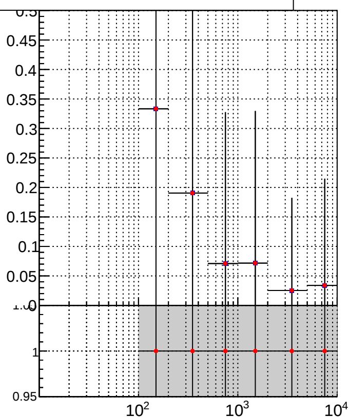
/data2/legianni/JSON-bkwd-fwd/no-modif/CMSSW_13_0_X_2023-01-24-1100/src/DQM_original DQM_modified
