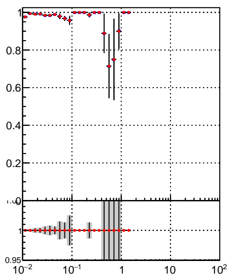
■ /data2/legianni/JSON-bkwd-fwd/no-modif/CMSW_13_0_X_2023-01-24-1100/src/DQM_original ● DQM_modified
