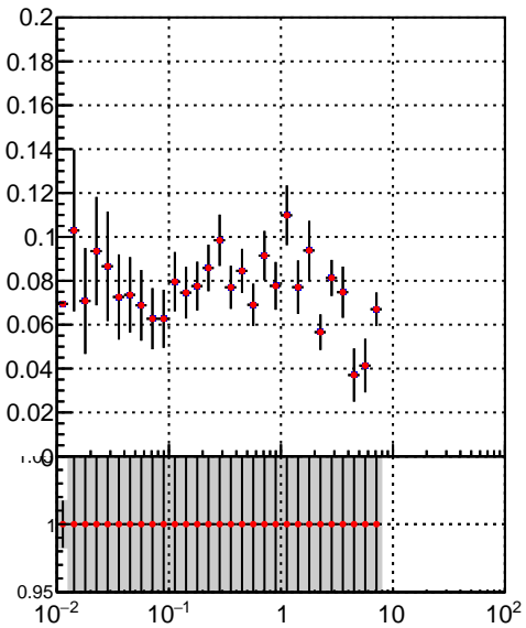
■ /data2/legianni/JSON-bkwd-fwd/no-modif/CMSW_13_0_X_2023-01-24-1100/src/DQM_original ● DQM_modified
