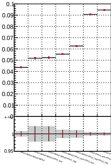
Fake rate vs. /data2/legianni/JSON-bkwd-fwd/no-modif/CMSSW_13_0_X_2023-01-24-1100/src/DQM_original DQM_modified
