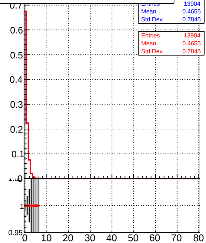
/data2/legianni/JSON-bkwd-fwd/no-modif/CMSSW_13_0_X_2023-01-24-1100/src/DQM_original DQM_modified
