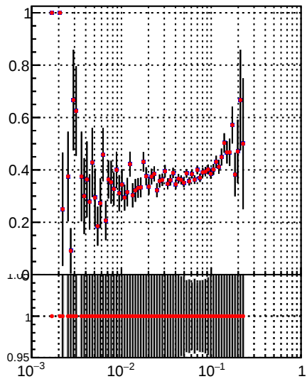
— /data2/legianni/JSON-bkwd-fwd/no-modif/CMSSW_13_0_X_2023-01-24-1100/src/DQM_original — DQM_modified
