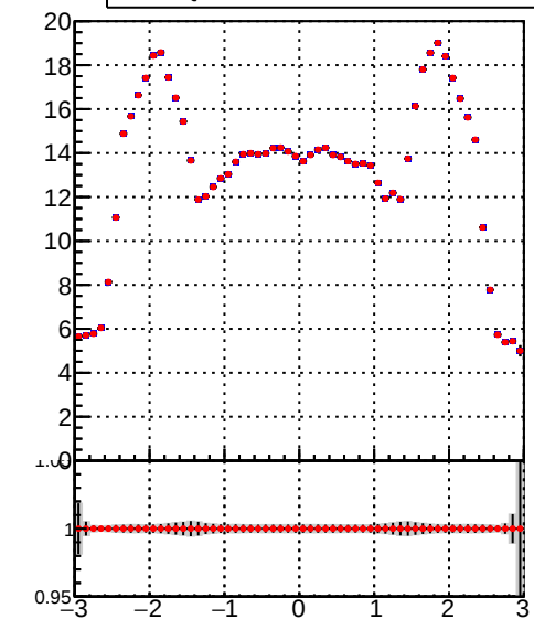
mean hit — /data2/legianni/JSON-bkwd-fwd/no-modif/CMSSW_13_0_X_2023-01-24-1100/src/DQM_original — DQM_modified
