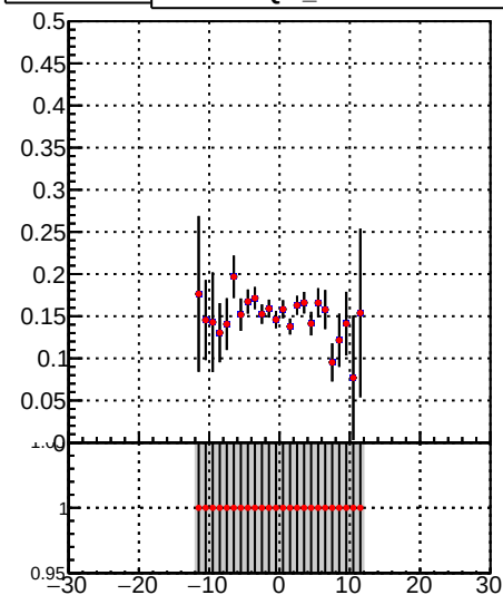
Fake rate vs verpos —●— /data2/legianni/JSON-bkwd-fwd/no-modif/CMSSW_13_0_X_2023-01-24-1100/src/DQM_original —●— DQM_modified
