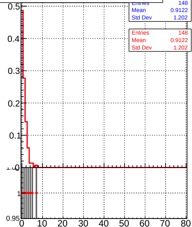
/data2/legianni/JSON-bkwd-fwd/no-modif/CMSSW_13_0_X_2023-01-24-1100/src/DQM_original DQM_modified
