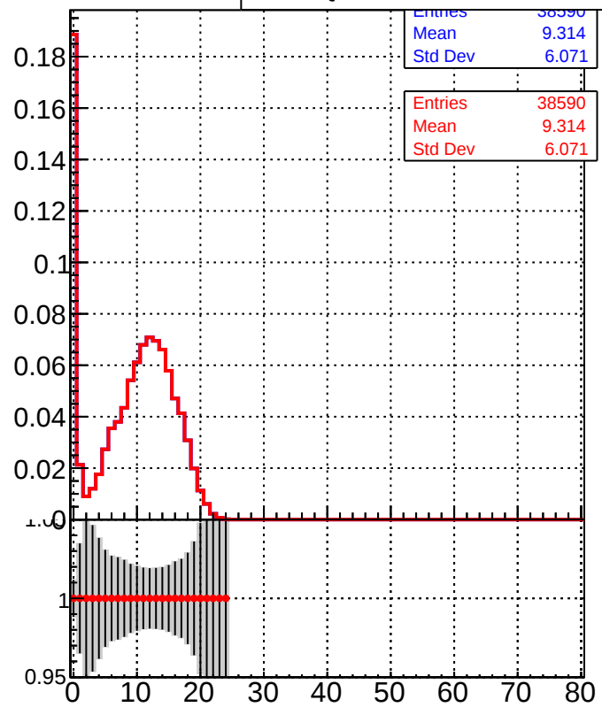
/data2/legianni/JSON-bkwd-fwd/no-modif/CMSSW_13_0_X_2023-01-24-1100/src/DQM_original DQM_modified
