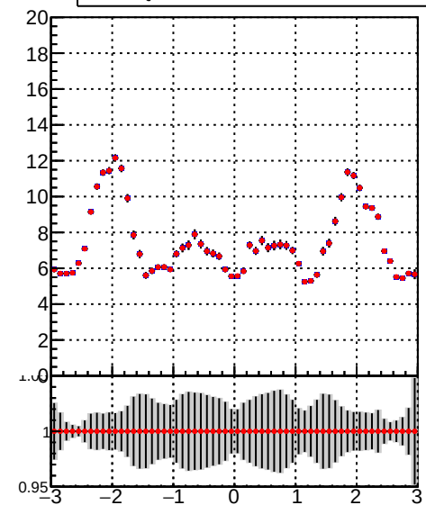
/data2/legianni/JSON-bkwd-fwd/no-modif/CMSSW_13_0_X_2023-01-24-1100/src/DQM_original DQM_modified
