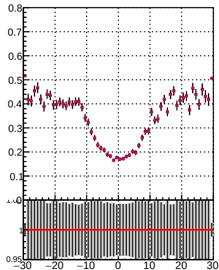
— /data2/legianni/JSON-bkwd-fwd/no-modif/CMSSW_13_0_X_2023-01-24-1100/src/DQM_original • DQM_modified
