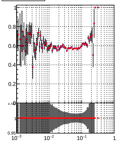
—•— /data2/legianni/JSON-bkwd-fwd/no-modif/CMSSW_13_0_X_2023-01-24-1100/src/DQM_original —•— DQM_modified
