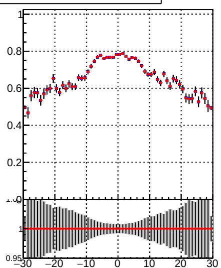
/data2/legianni/JSON-bkwd-fwd/no-modif/CMSSW_13_0_X_2023-01-24-1100/src/DQM_original Fake rate vs vertpos DQM_modified
