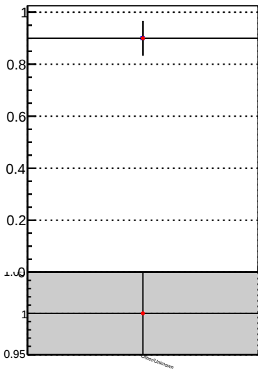
Fake rate vs. /data2/legianni/JSON-bkwd-fwd/no-modif/CMSSW_13_0_X_2023-01-24-1100/src/DQM_original DQM_modified
