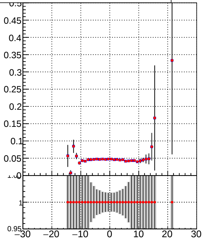
— /data2/legianni/JSON-bkwd-fwd/no-modif/CMSSW_13_0_X_2023-01-24-1100/src/DQM_original —• DQM_modified
