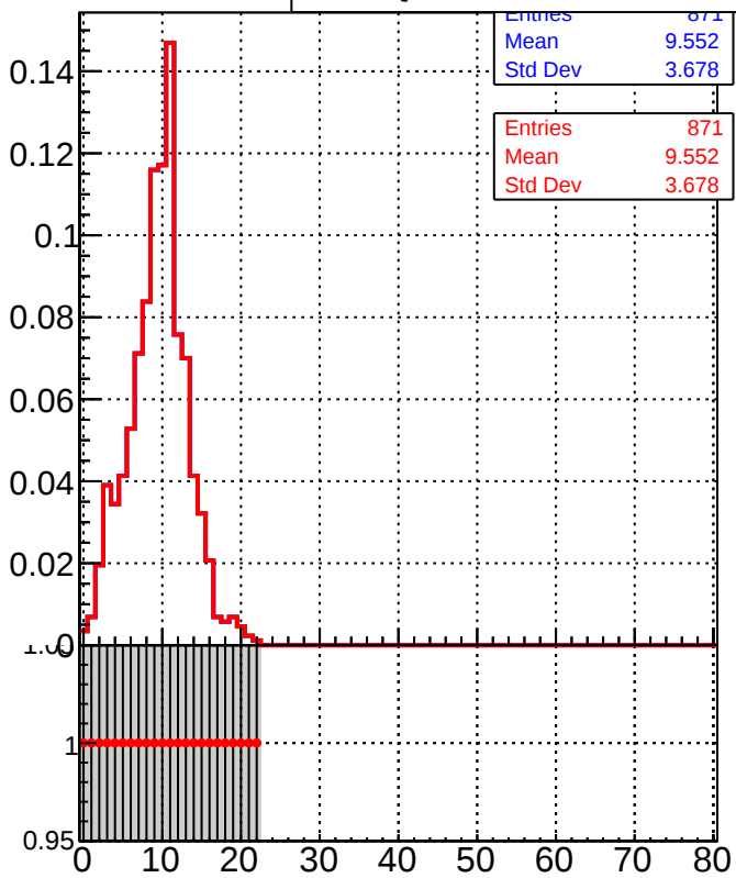
Legend: /data2/legianni/JSON-bkwd-fwd/no-modif/CMSSW_13_0_X_2023-01-24-1100/src/DQM_original (grey bars), DQM_modified (red line with dots)
