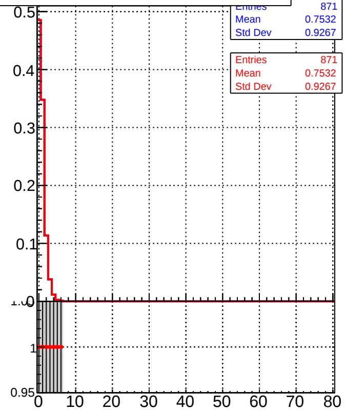
Legend: /data2/legianni/JSON-bkwd-fwd/no-modif/CMSSW_13_0_X_2023-01-24-1100/src/DQM_original (grey bars), DQM_modified (red line with dots)
