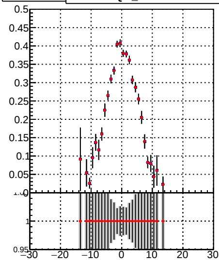
Fake rate vs v —●— /data2/legianni/JSON-bkwd-fwd/no-modif/CMSSW_13_0_X_2023-01-24-1100/src/DQM_original —●— DQM_modified
