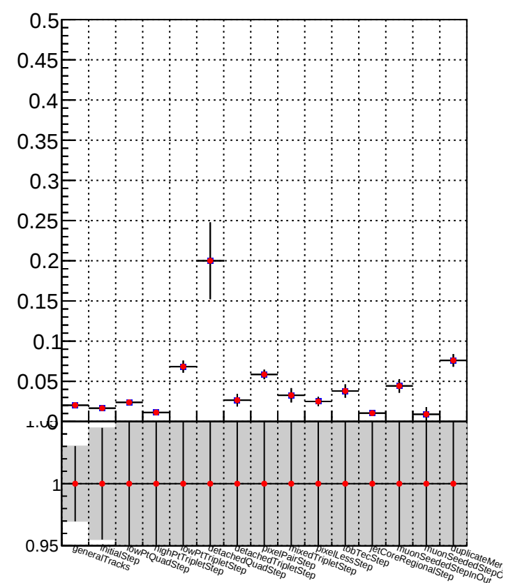
/data2/legianni/JSON-bkwd-fwd/no-modif/CMSSW_13_0_X_2023-01-24-1100/src/DQM_original DQM_modified
