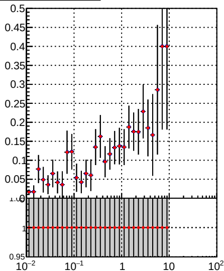
/data2/legianni/JSON-bkwd-fwd/no-modif/CMSSW_13_0_X_2023-01-24-1100/src/DQM_original DQM_modified
