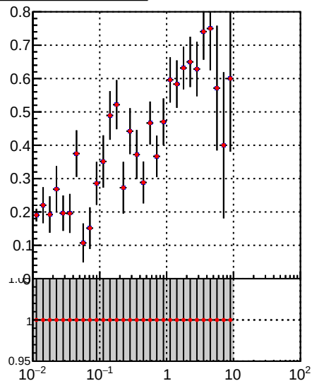
/data2/legianni/JSON-bkwd-fwd/no-modif/CMSSW_13_0_X_2023-01-24-1100/src/DQM_original DQM_modified
