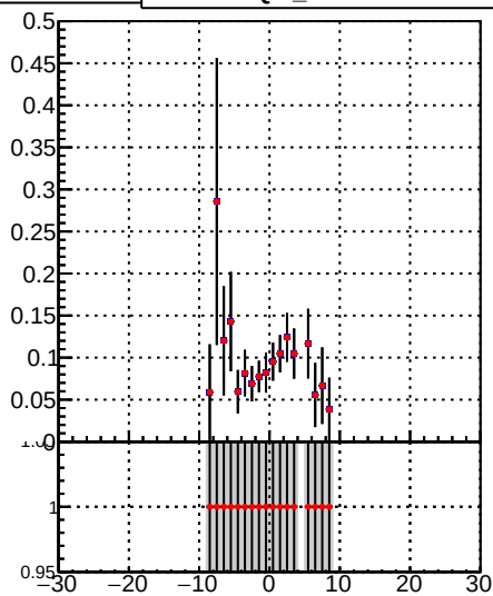
/data2/legianni/JSON-bkwd-fwd/no-modif/CMSSW_13_0_X_2023-01-24-1100/src/DQM_original DQM_modified
