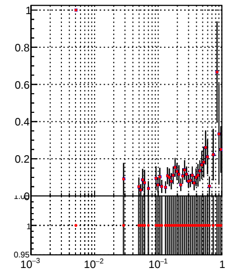
Legend: /data2/legianni/JSON-bkwd-fwd/no-modif/CMSSW_13_0_X_2023-01-24-1100/src/DQM_original (blue line), DQM_modified (red line)
