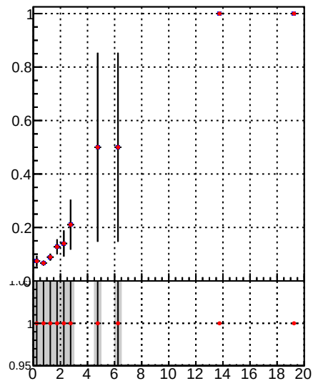
Fake rate vs. /data2/legianni/JSON-bkwd-fwd/no-modif/CMSSW_13_0_X_2023-01-24-1100/src/DQM_original DQM_modified
