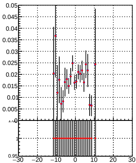
Fake rate vs d
