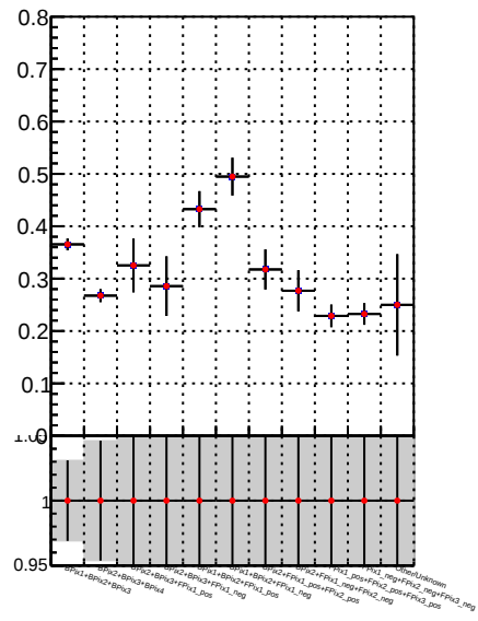
Fake rate vs. —•— /data2/legianni/JSON-bkwd-fwd/no-modif/CMSSW_13_0_X_2023-01-24-1100/src/DQM_original -•- DQM_modified
