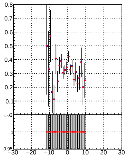
— /data2/legianni/JSON-bkwd-fwd/no-modif/CMSSW_13_0_X_2023-01-24-1100/src/DQM_original — DQM_modified
