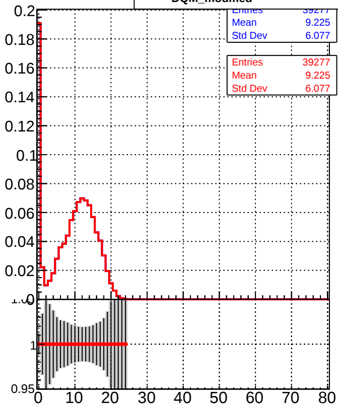
- /data2/legianni/JSON-bkwd-fwd/no-modif/CMSSW_13_0_X_2023-01-24-1100/src/DQM_original - DQM_modified
