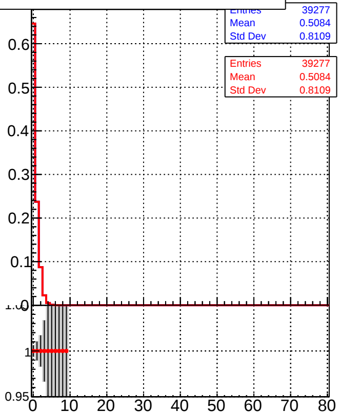
- /data2/legianni/JSON-bkwd-fwd/no-modif/CMSSW_13_0_X_2023-01-24-1100/src/DQM_original - DQM_modified
