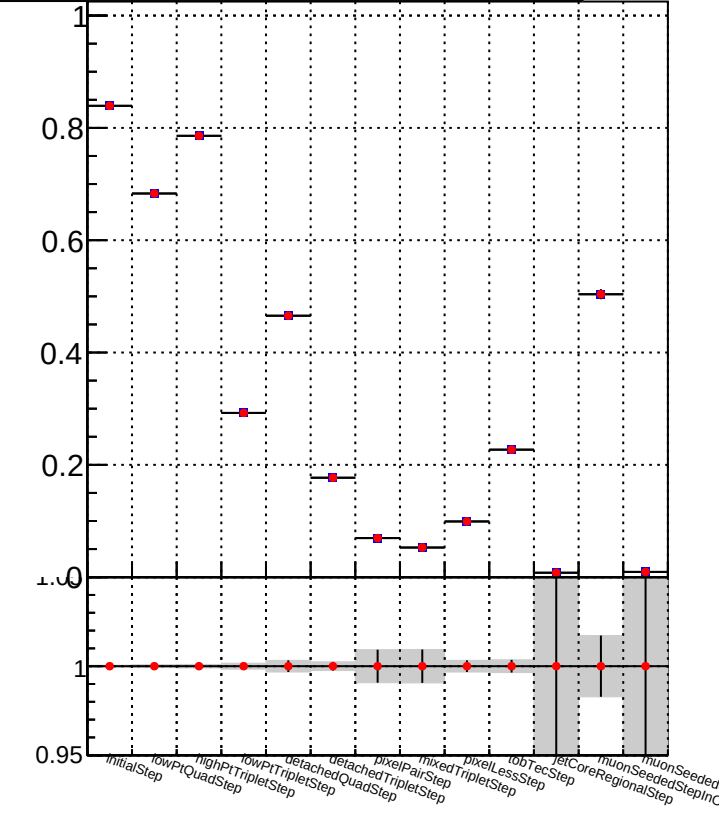
Duplicates rate vs collection Legend: - /data2/legianni/JSON-bkwd-fwd/no-modif/CMSSW_13_0_X_2023-01-24-1100/src/DQM_original (grey square) - DQM_modified (red circle)
