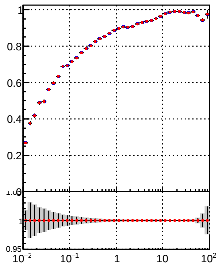
/data2/legianni/JSON-bkwd-fwd/no-modif/CMSSW_13_0_X_2023-01-24-1100/src/DQM_original Fake rate vs v DQM_modified
