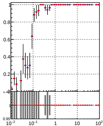
Fake rate vs vertpos Legend: - /data2/legianni/JSON-bkwd-fwd/no-modif/CMSSW_13_0_X_2023-01-24-1100/src/DQM_original - DQM_modified
