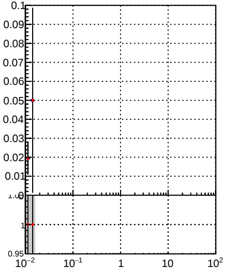
Fake rate vs vertpos Legend: - /data2/legianni/JSON-bkwd-fwd/no-modif/CMSSW_13_0_X_2023-01-24-1100/src/DQM_original - DQM_modified
