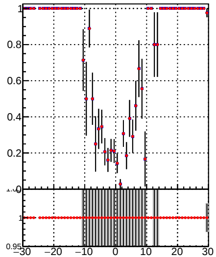
Fake rate vs vertpos Legend: - /data2/legianni/JSON-bkwd-fwd/no-modif/CMSSW_13_0_X_2023-01-24-1100/src/DQM_original - DQM_modified
