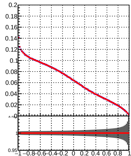
Fake rate vs. MVA1
