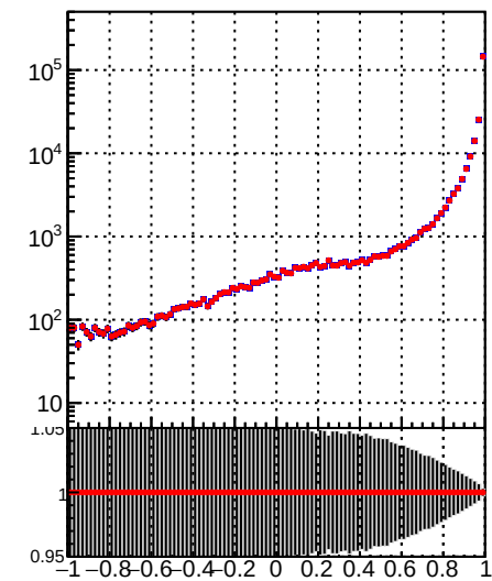
N of associated tracks (recoToSim) vs. MVA1
