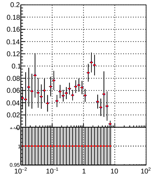
Efficiency vs vertpos Legend: \square /data2/legianni/JSON-bkwd-fwd/no-modif/CMSSW_13_0_X_2023-01-24-1100/src/DQM_original \bullet DQM_modified
