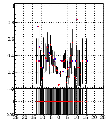
Efficiency vs DQM_modified
