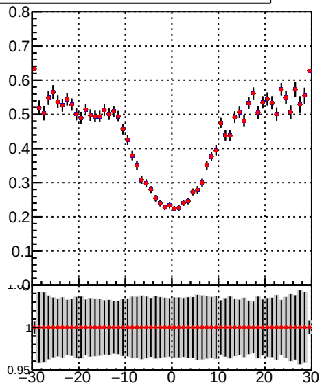
Efficiency vs vertpos Legend: - /data2/legianni/JSON-bkwd-fwd/no-modif/CMSSW_13_0_X_2023-01-24-1100/src/DQM_original (blue line with dots) - DQM_modified (red line with dots)
