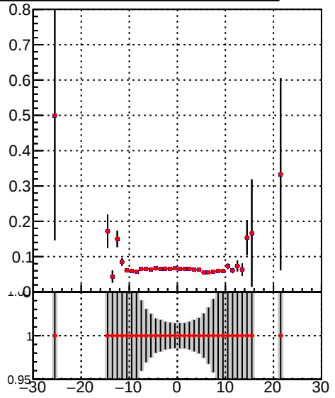
Efficiency vs. sim PV z — /data2/legianni/JSON-bkwd-fwd/no-modif/CMSW_13_0_X_2023-01-24-1100/src/DQM_original — DQM_modified
