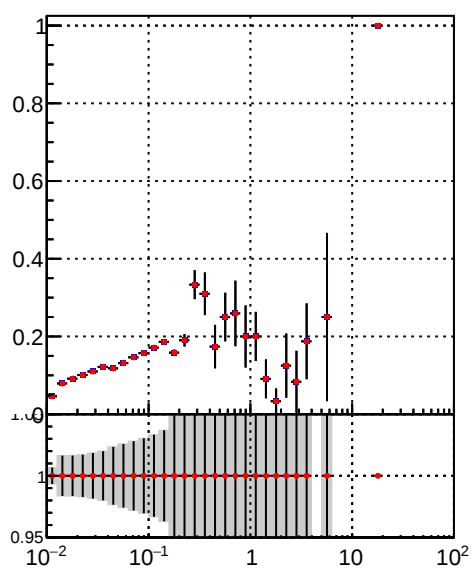
Efficiency vs. sim PV z — /data2/legianni/JSON-bkwd-fwd/no-modif/CMSW_13_0_X_2023-01-24-1100/src/DQM_original — DQM_modified
