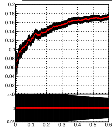
Fake rate Legend: — /data2/legianni/JSON-bkwd-fwd/no-modif/CMSSW_13_0_X_2023-01-24-1100/src/DQM_original — DQM_modified
