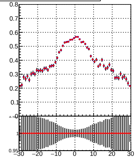
—•— /data2/legianni/JSON-bkwd-fwd/no-modif/CMSSW_13_0_X_2023-01-24-1100/src/DQM_original —•— DQM_modified
