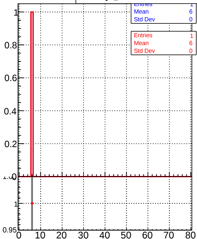
/data2/legianni/JSON-bkwd-fwd/no-modif/CMSSW_13_0_X_2023-01-24-1100/src/DQM_original DQM_modified
