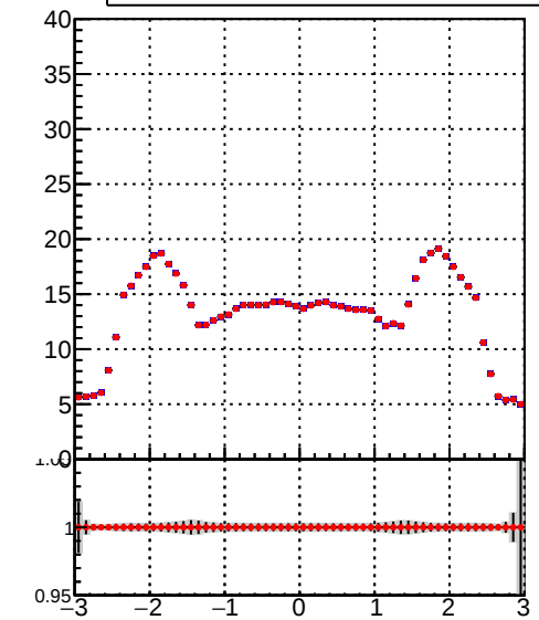
mean hit — /data2/legianni/JSON-bkwd-fwd/no-modif/CMSSW_13_0_X_2023-01-24-1100/src/DQM_original — DQM_modified
