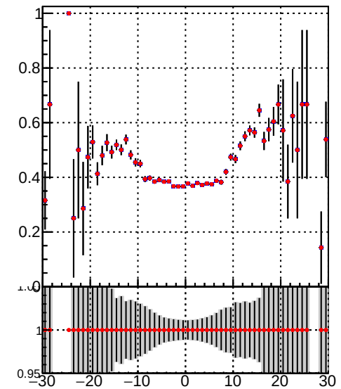
— /data2/legianni/JSON-bkwd-fwd/no-modif/CMSW_13_0_X_2023-01-24-1100/src/DQM_original — DQM_modified
