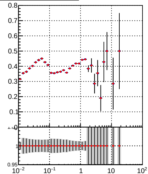
— /data2/legianni/JSON-bkwd-fwd/no-modif/CMSW_13_0_X_2023-01-24-1100/src/DQM_original — DQM_modified
