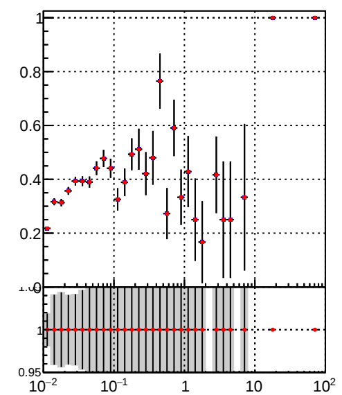
— /data2/legianni/JSON-bkwd-fwd/no-modif/CSSW_13_0_X_2023-01-24-1100/src/DQM_original — DQM_modified
