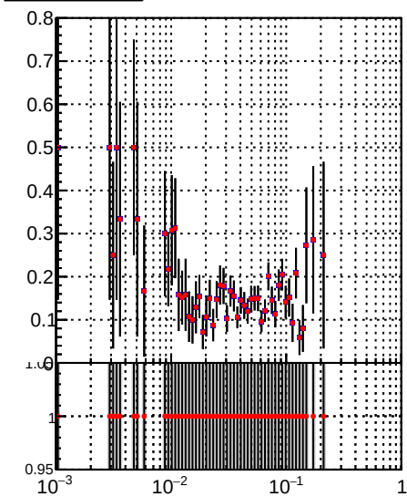
—•— /data2/legianni/JSON-bkwd-fwd/no-modif/CMSSW_13_0_X_2023-01-24-1100/src/DQM_original —•— DQM_modified
