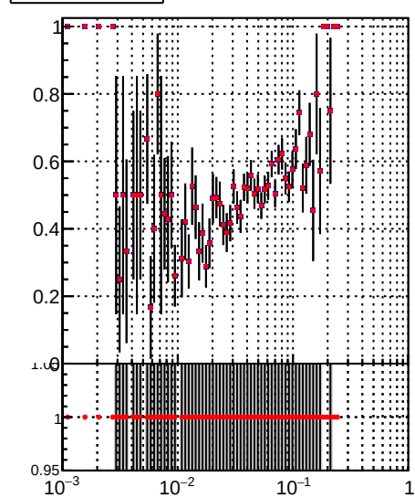
—•— /data2/legianni/JSON-bkwd-fwd/no-modif/CMSSW_13_0_X_2023-01-24-1100/src/DQM_original —•— DQM_modified
