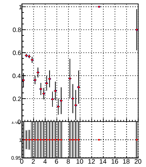
Fake rate vs. - /data2/legianni/JSON-bkwd-fwd/no-modif/CMSSW_13_0_X_2023-01-24-1100/src/DQM_original - DQM_modified
