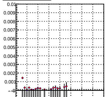
Duplicates Rate vs hit
