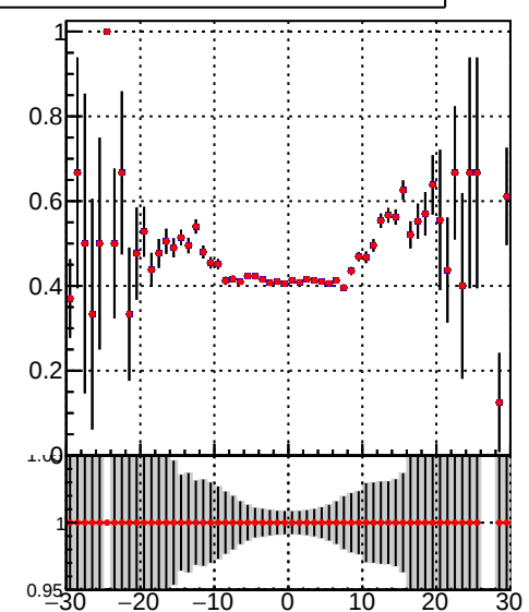
Efficiency vs vertpos Legend: - /data2/legianni/JSON-bkwd-fwd/no-modif/CMSW_13_0_X_2023-01-24-1100/src/DQM_original (blue line with dots) - DQM_modified (red line with dots)
