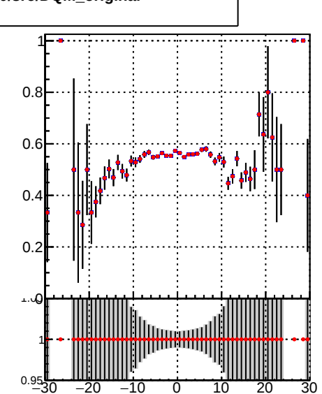
—•— /data2/legianni/JSON-bkwd-fwd/no-modif/CMSSW_13_0_X_2023-01-24-1100/src/DQM_original —•— DQM_modified
