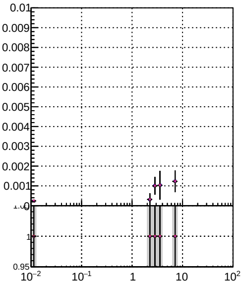
Efficiency Legend: DOM modified DOM modified_PL DOM modified_PL_New1 DOM modified_PL_New2 Path: /data2/legami/JSON-bkwd-fwd/mo-modif/CMSSW_13_0_X_2023-01-24_1100/src/DQM_original
