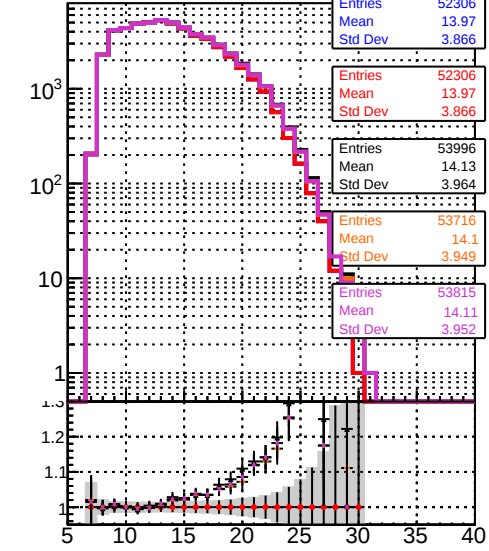
mean hit Legend: data2/legami, JSON-bkwd-fwd/no-modif/CMSW_13_0_X_2023-01-24-1100/src/DQM_original, DQM modified PL, DQM modified PL New1, DQM modified PL New2
