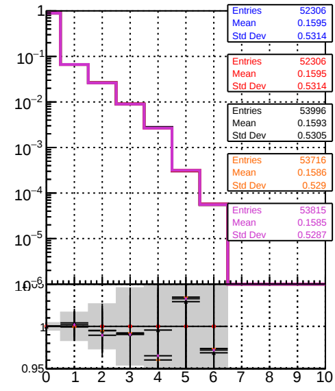
mean hit Legend: data2/legami, JSON-bkwd-fwd/no-modif/CMSW_13_0_X_2023-01-24-1100/src/DQM_original, DQM modified PL, DQM modified PL New1, DQM modified PL New2
